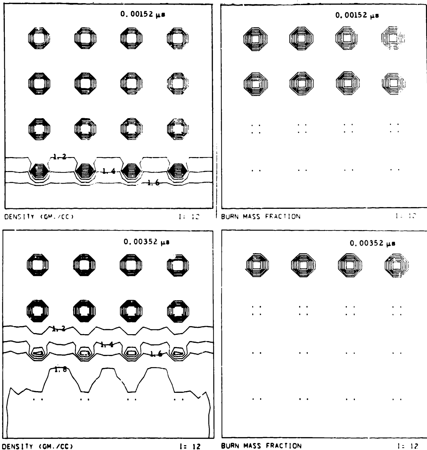
Fig. 5. The cross sections for the 12th cell in the x-direction for the interaction of a 5.5-GPa shock for 1.6 \times 10^{-3} \mu\text{s} followed by an 8.5-GPa shock in a 0.028-mm cube of nitromethane with ninety-one 0.002-mm cubical holes. The interval between isopycnics is 0.2 \text{ mg/mm}^3 and between burn fraction is 0.2. Shows desensitization by preshocking.
